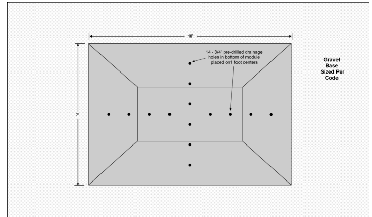
View 3: Pad Disposal Top View
