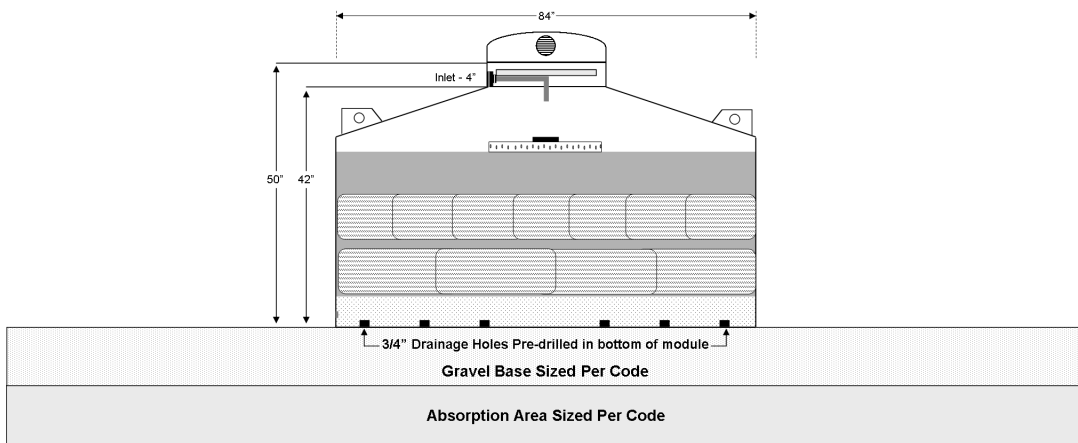
View 2: Cross Section, Width
