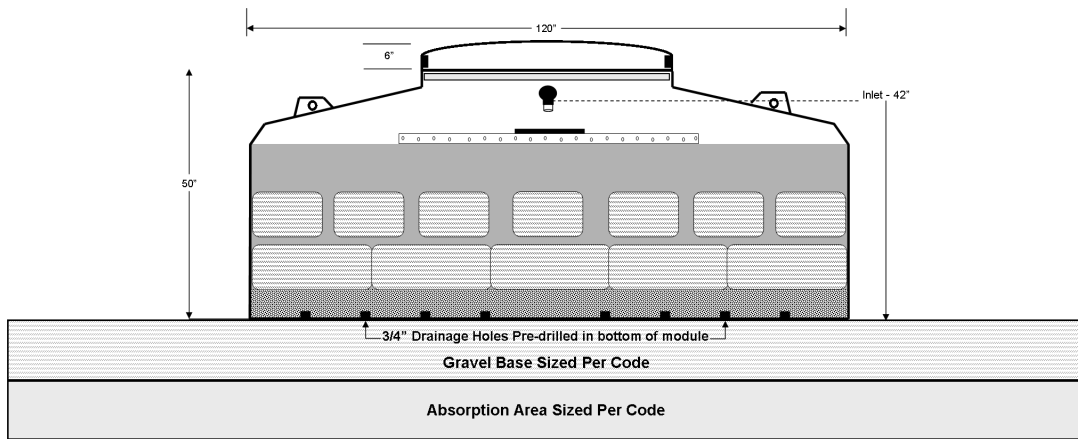
View 1: Cross Section, Length
