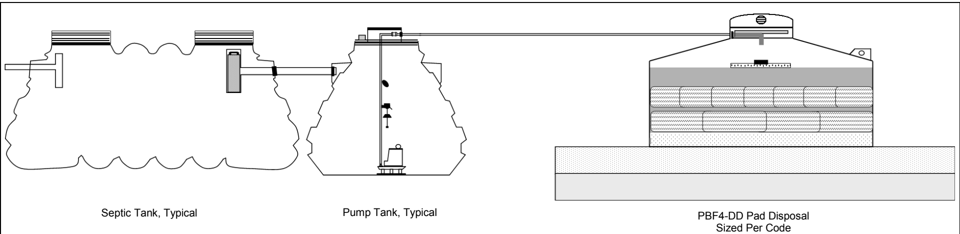
View 1: PBF4-DD Pad Disposal Layout
