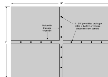
View 4: PBF4-DD Module Bottom
