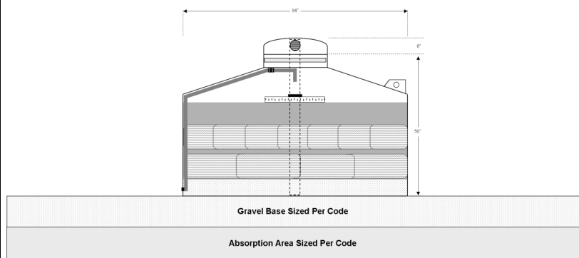
View 2: PBF4-P-DD Cross Section Pad Disposal
