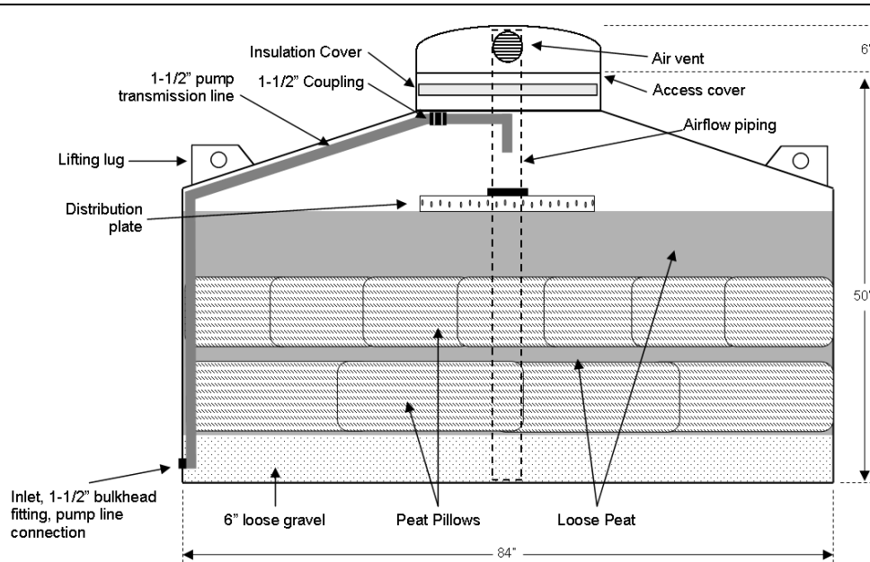
View 1: PBF4-P-DD Cross Section View, Width
