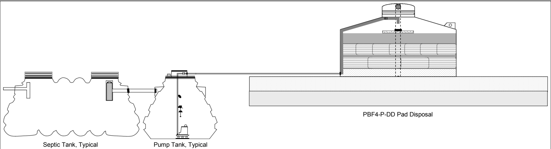
View 1: PBF4-P-DD Pad Disposal Layout
