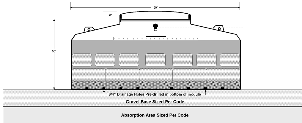
View 2: Module Dimensions, Length
