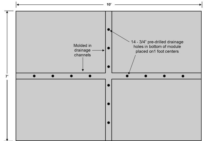
View 3: PBF4-DD Module Bottom
