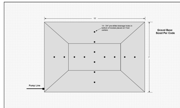
View 3: PBF4-P-DD Pad Disposal, Top
